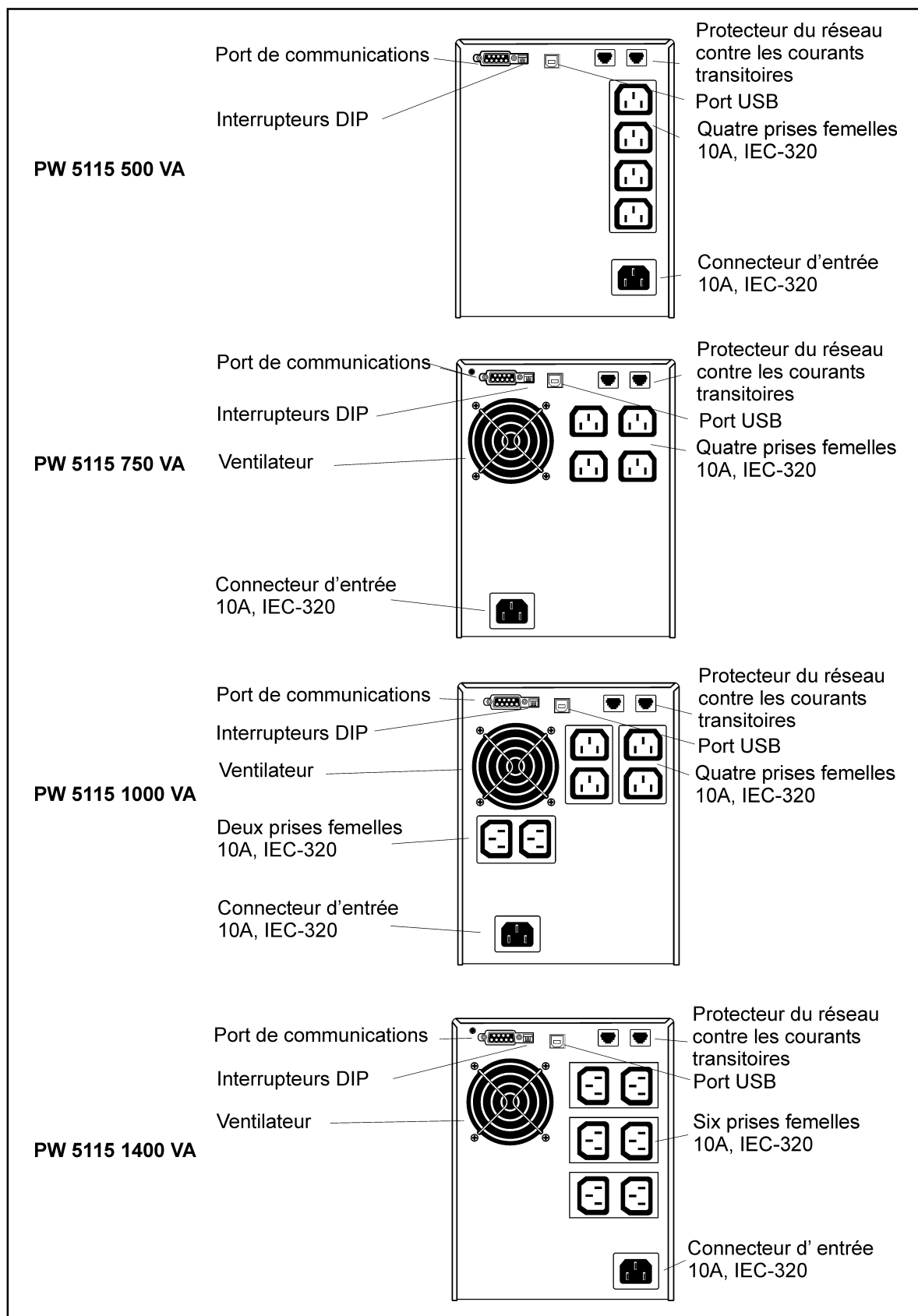
Figure 3. Panneaux arrières
